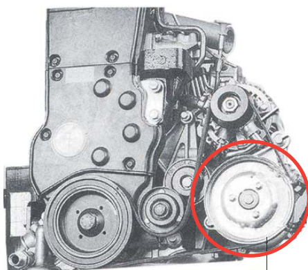
Steering pump (12)
