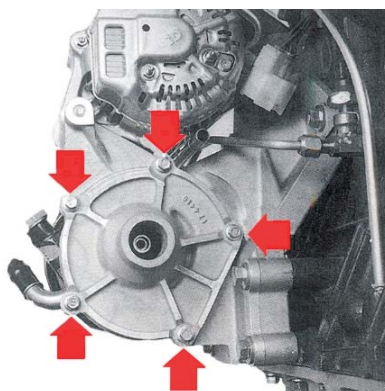
Water pump bolts
