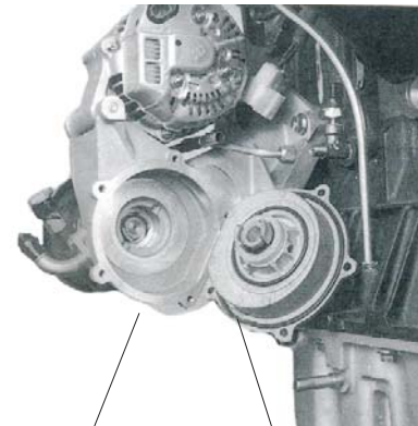
Water pump
